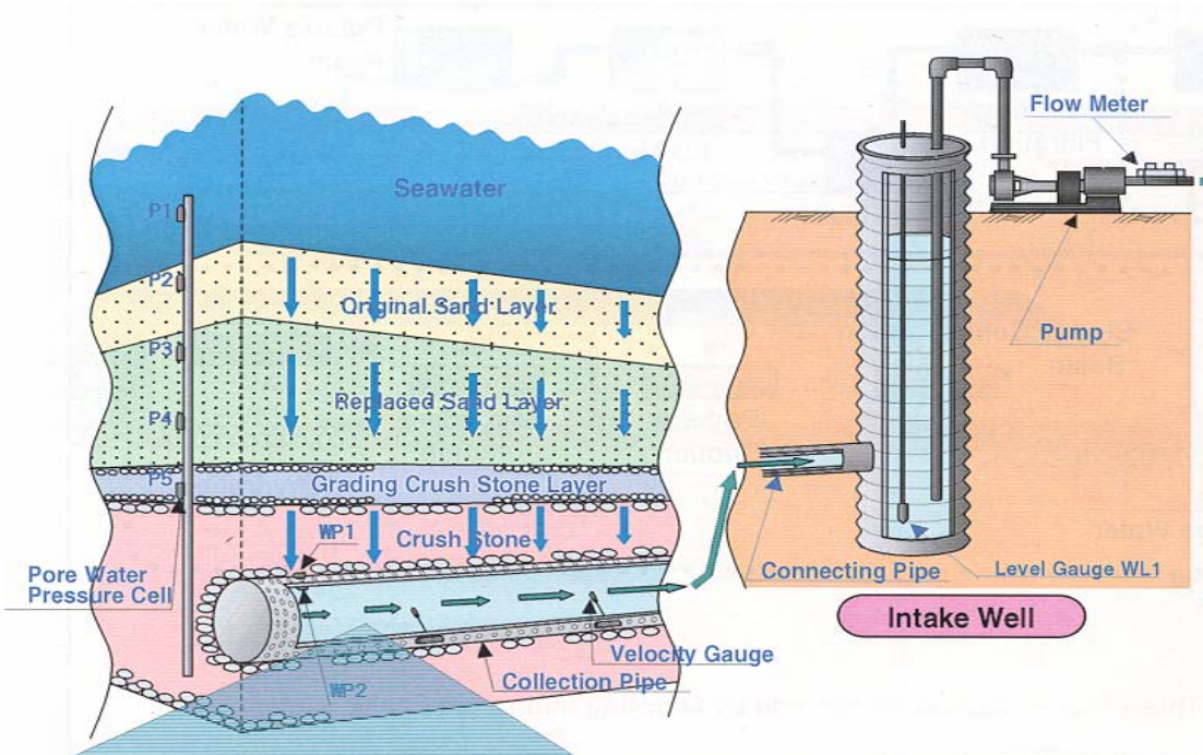
Figure 4-5 – A Cross-Section of Subsurface Infiltration Gallery
